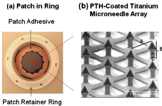
Fig. 1 Transdermal microprojection patch delivery system— a. ZP-PTH patch/retainer ring; The titanium microneedle array is 2 cm 2 in area and attached to a 5 cm 2 adhesive with backing. The adhesive is attached to a polycarbonate ring with 4 scored tabs. b. SEM of PTH (1-34)-coated microprojection array: A) distance between microneedles: 370microns; B) length from microneedle tip to base plate: 190 microns; C) shaft width: 60 microns. The PTH (1-34) formulation coating is restricted to the arrowhead area of the microneedle. The tip angle is 60 degrees and distance from tip to arrowhead base is 100 microns.
